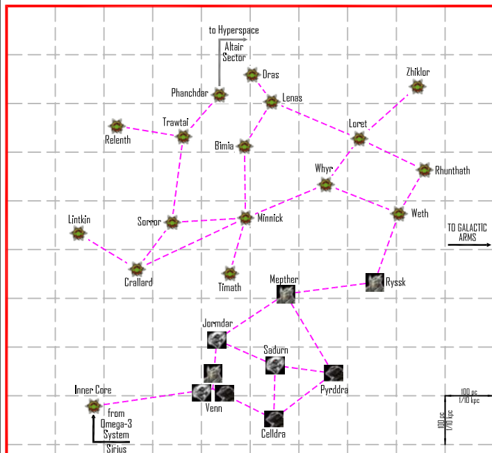
MILKY WAY GALAXY - GALACTIC CENTER - INNER CORE SECTOR
