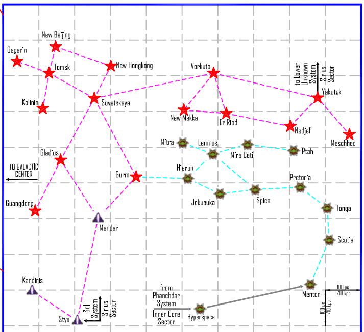
MILKY WAY GALAXY - ORION ARM - ALTAIR SECTOR
