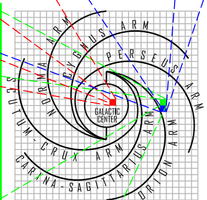
MILKY WAY GALAXY - ORION ARM - ALTAIR SECTOR
